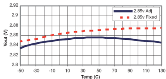
Fig. 12: V_{IN}=4.85V , I_{OUT}=10mA
